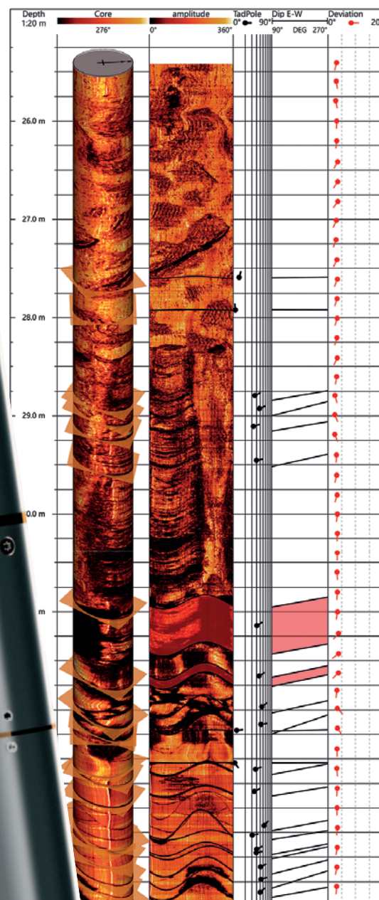
The High Resolution Acoustic Televiewer (HRAT) ® Probe, with logging data example
