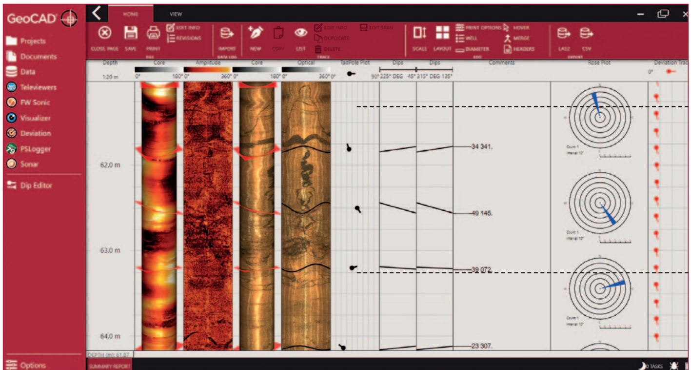
Example TelevIEWER data processed using GeoCAD® software from Robertson Geo.
